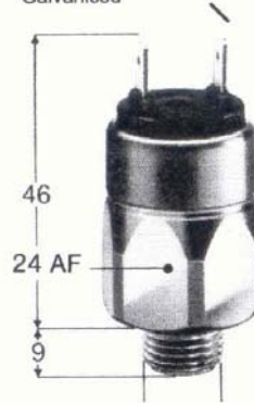
Pressure Switch
